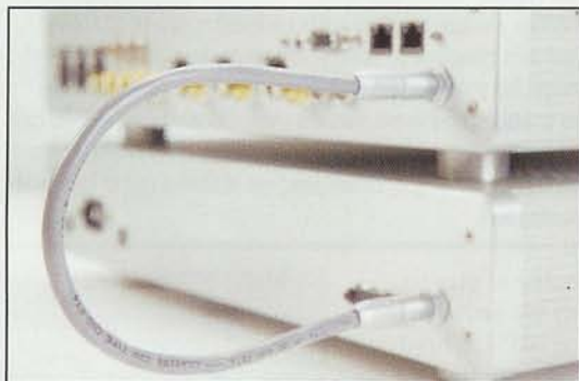
Above: Evolution Two inputs labelled only as S1-4, B1-3 and C1-3 on the panel (single-ended/balanced/CAST), but can be assigned pre-set names for the fluorescent display like 8TRK, DCC, GAME and HI-8; [left] unlike power amp, power connection from PSU to pre-amp is by cable
