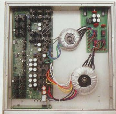
Evolution Two pre-amp's power supply [above], with a sea of heatsinked regulators
