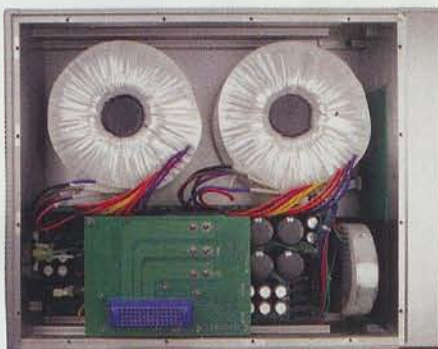
Power supply for Evolution One power amp
