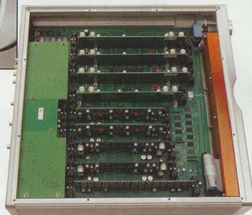
Evolution Two pre-amp: all inputs with JFET input buffer
